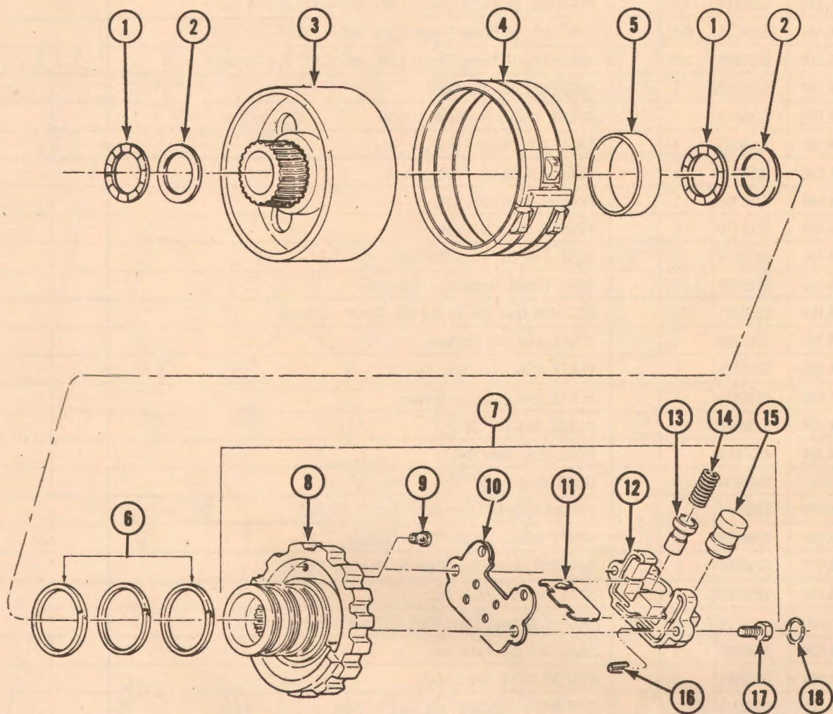
REACTION SUN GEAR AND GOVERNOR
